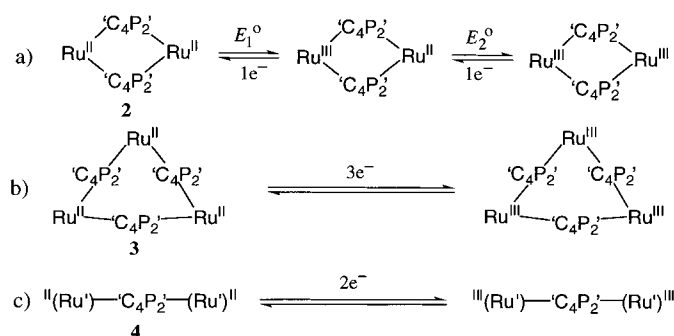
Scheme 1. Description of the redox behavior of 2–4 : \text{Ru} = [\text{RuCl}(\text{tpy})] , \text{Ru}' = [\text{RuCl}(\text{bpy})_2] , and ' \text{C}_4\text{P}_2 ' = \text{Ph}_2\text{P}-\text{C}\equiv\text{C}-\text{C}\equiv\text{C}-\text{PPh}_2 .
